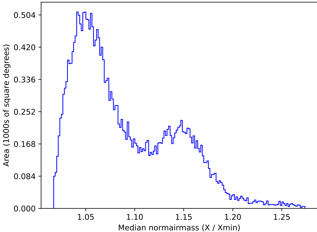
too_elab_r64_d3_gz_v3.4_10yrs All sky z band: Median normairmass
