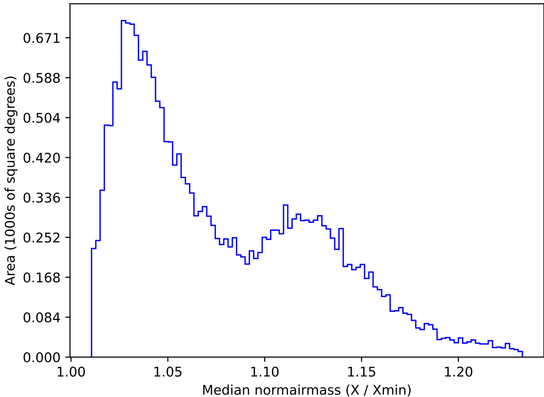
too_elab_r64_d3_gz_v3.4_10yrs All sky u band: Median normairmass
