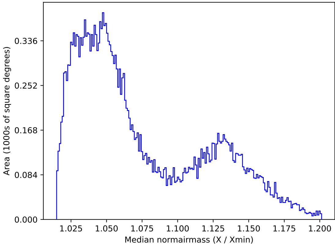
too_elab_r64_d3_gz_v3.4_10yrs All sky r band: Median normairmass
