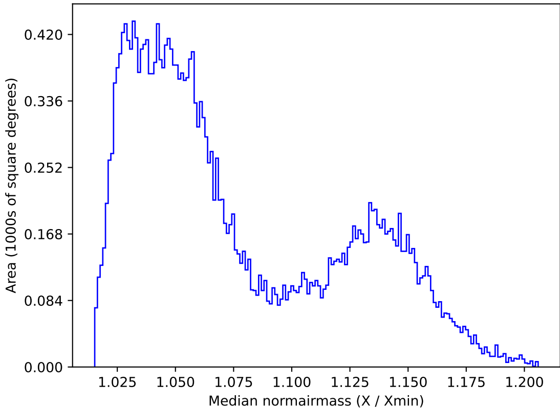
too_elab_r64_d3_gz_v3.4_10yrs All sky i band: Median normairmass
