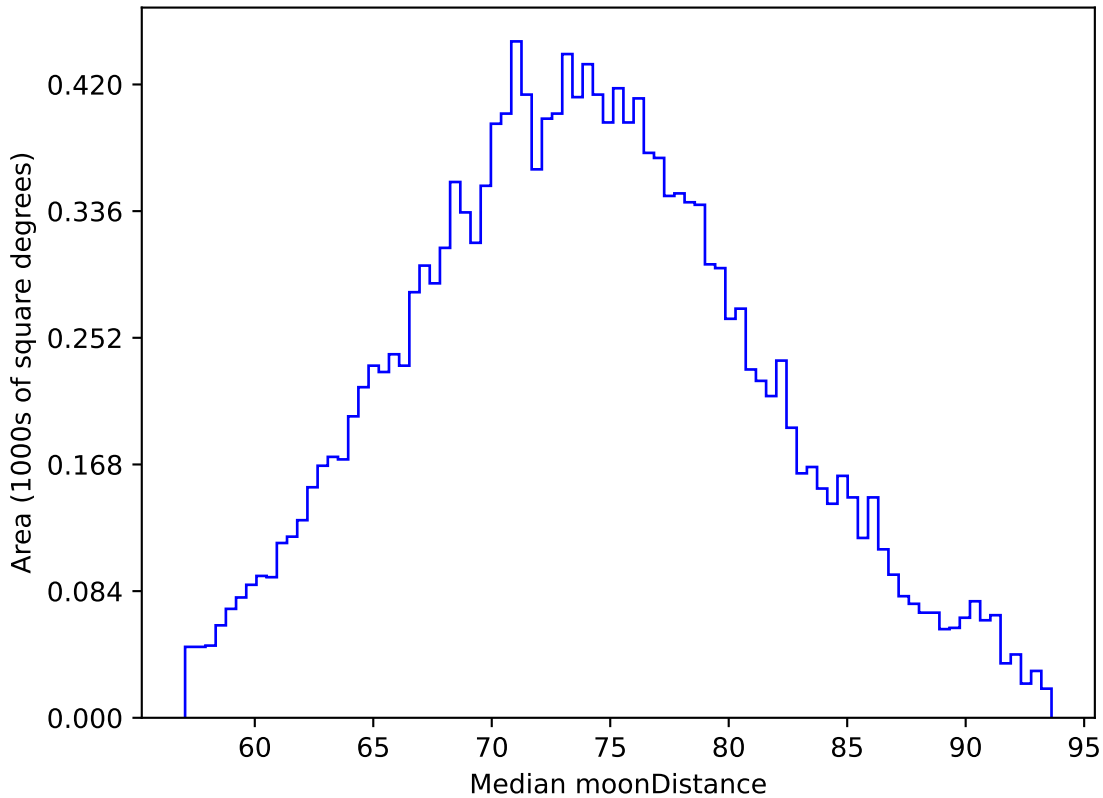
too_elab_r64_d3_gz_v3.4_10yrs WFD z band: Median moonDistance
