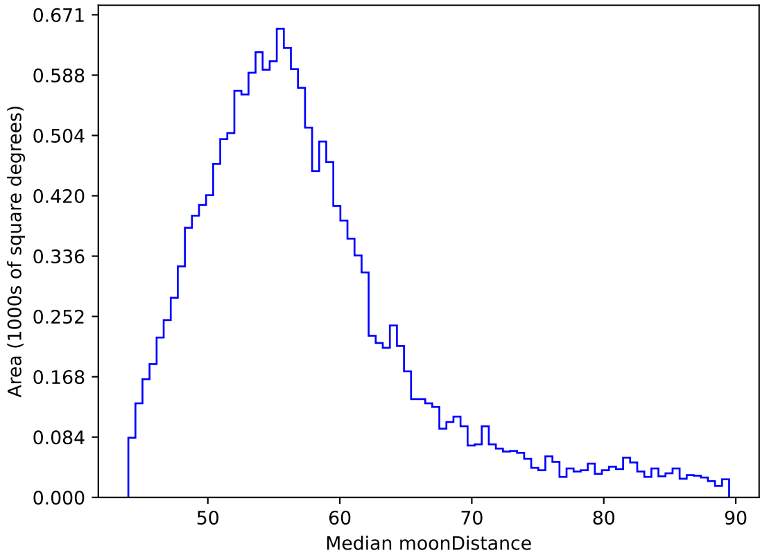
too_elab_r64_d3_gz_v3.4_10yrs WFD y band: Median moonDistance
