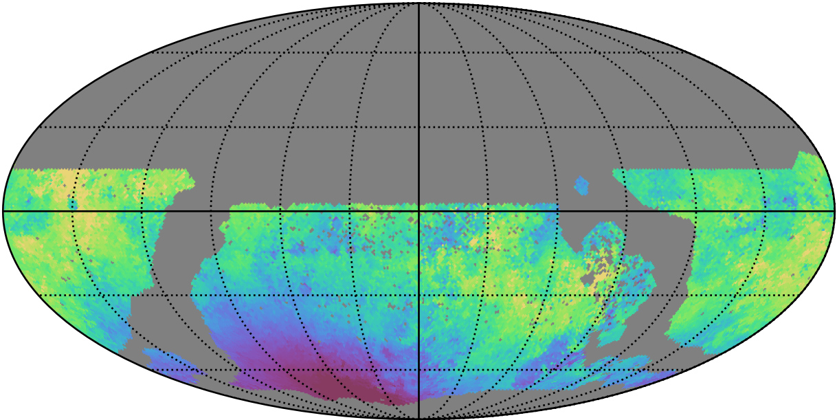
too_elab_r64_d3_gz_v3.4_10yrs WFD u band: Median moonDistance
