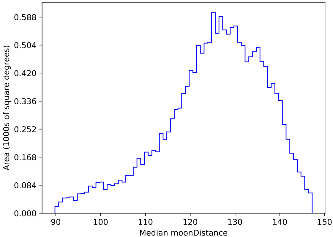
too_elab_r64_d3_gz_v3.4_10yrs WFD u band: Median moonDistance
