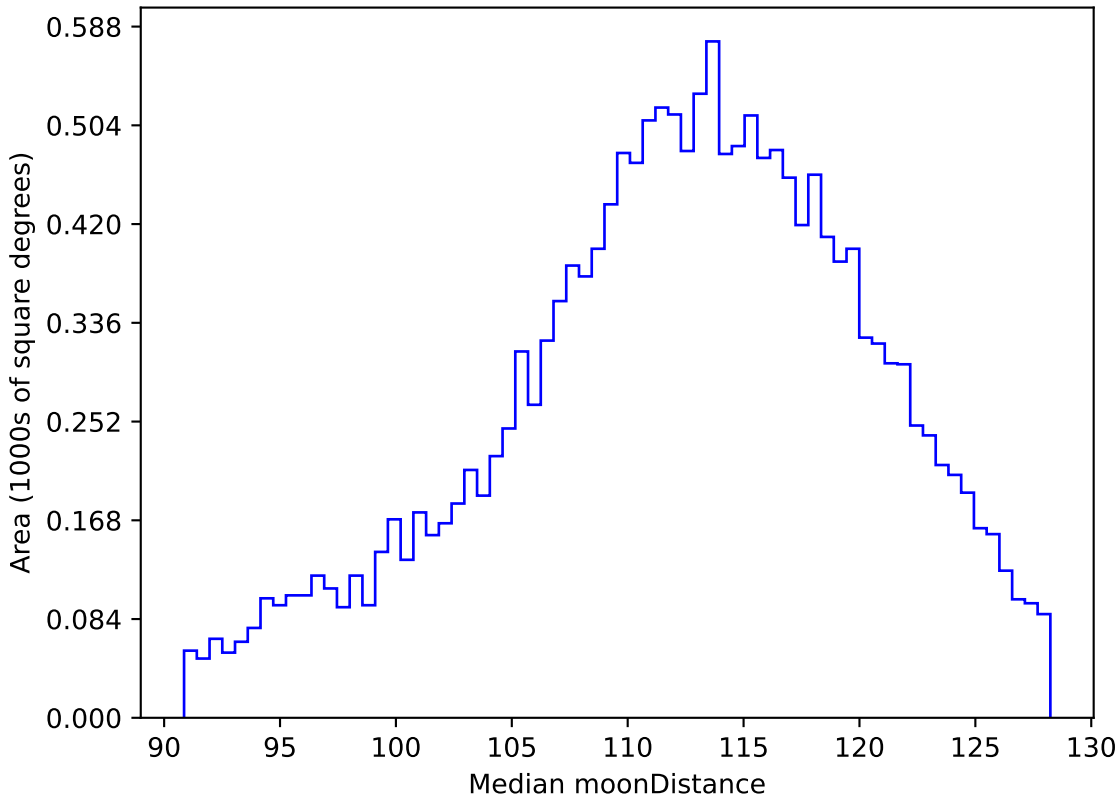
too_elab_r64_d3_gz_v3.4_10yrs WFD r band: Median moonDistance
