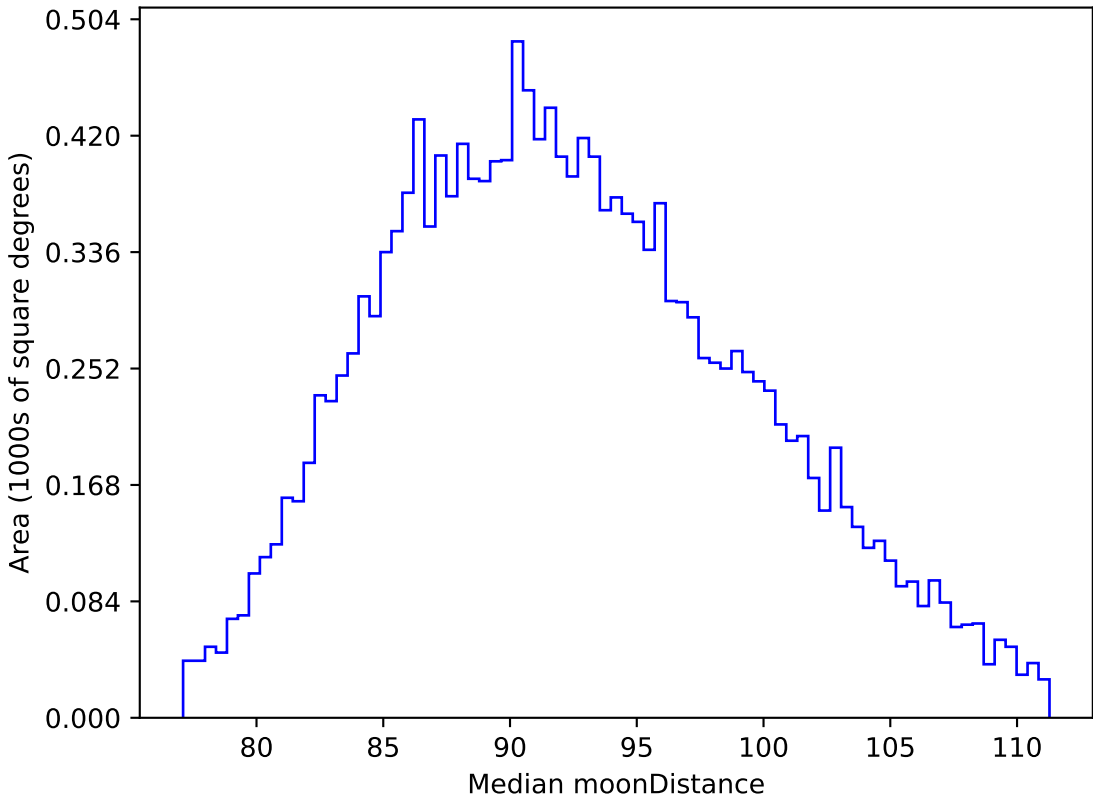
too_elab_r64_d3_gz_v3.4_10yrs WFD i band: Median moonDistance
