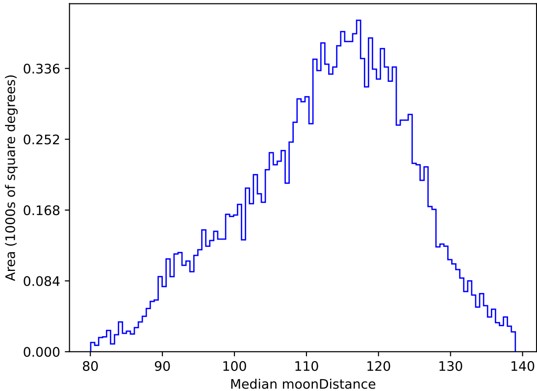
too_elab_r64_d3_gz_v3.4_10yrs WFD g band: Median moonDistance
