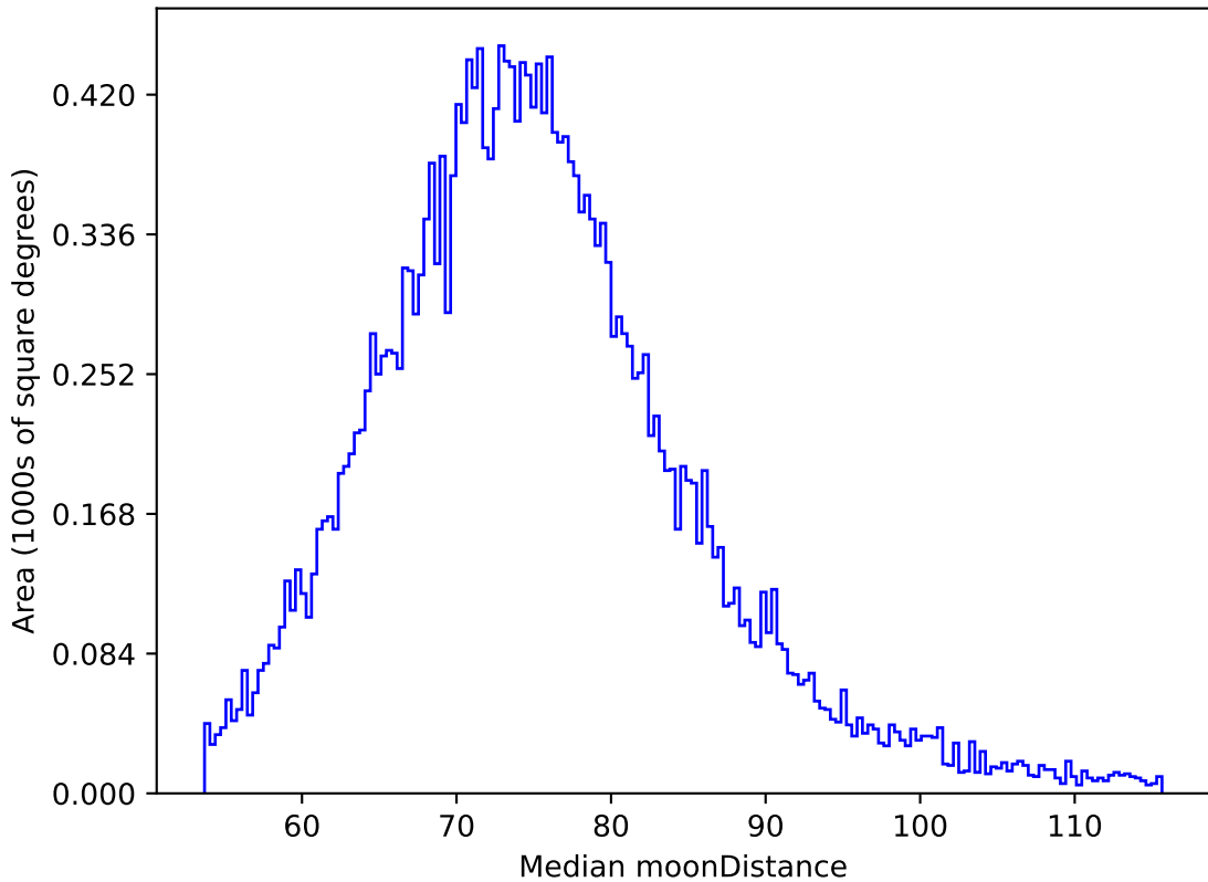
too_elab_r64_d3_gz_v3.4_10yrs All sky z band: Median moonDistance
