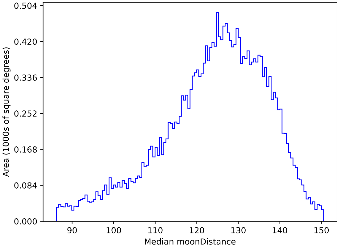
too_elab_r64_d3_gz_v3.4_10yrs All sky u band: Median moonDistance
