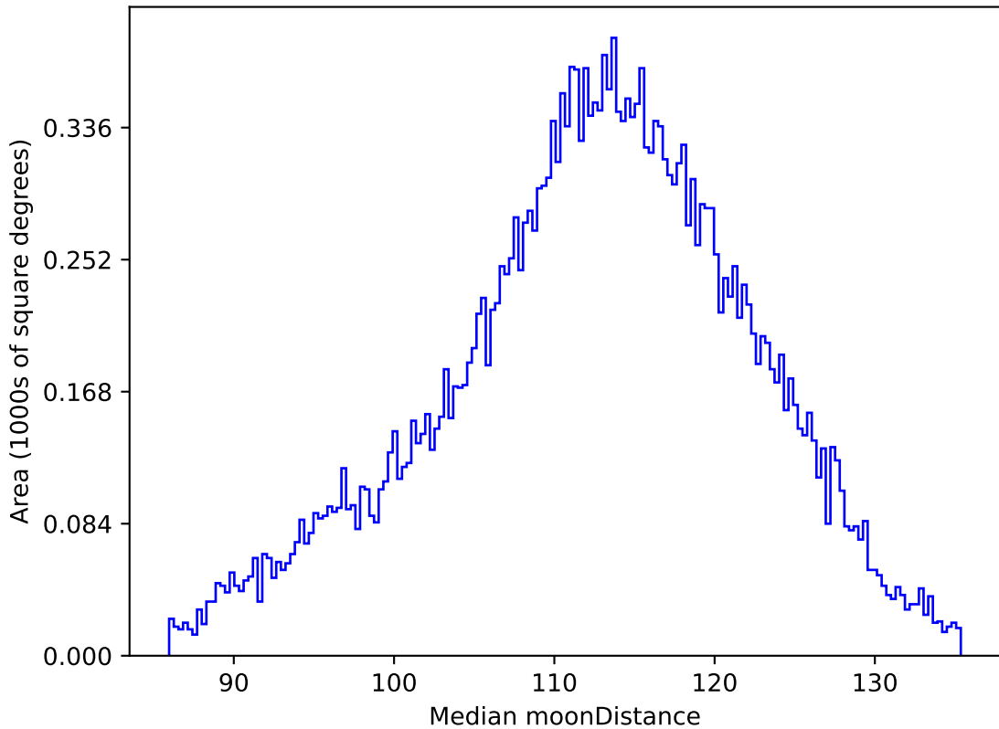
too_elab_r64_d3_gz_v3.4_10yrs All sky r band: Median moonDistance
