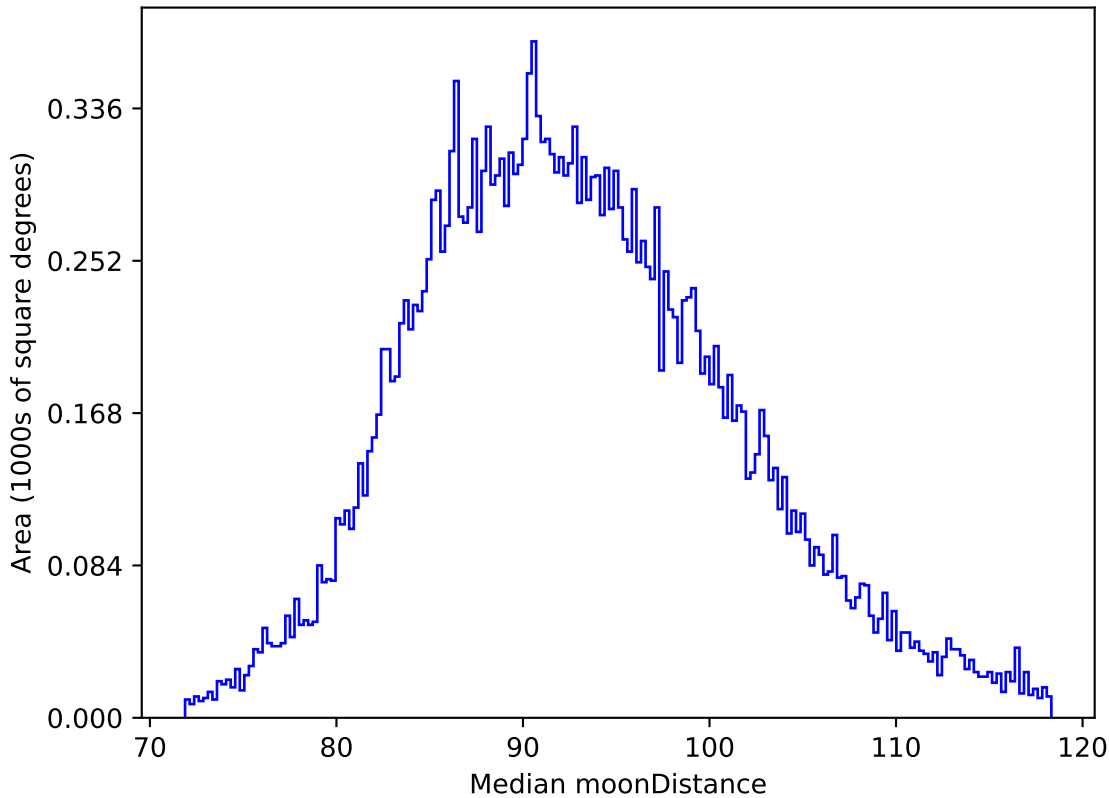
too_elab_r64_d3_gz_v3.4_10yrs All sky i band: Median moonDistance
