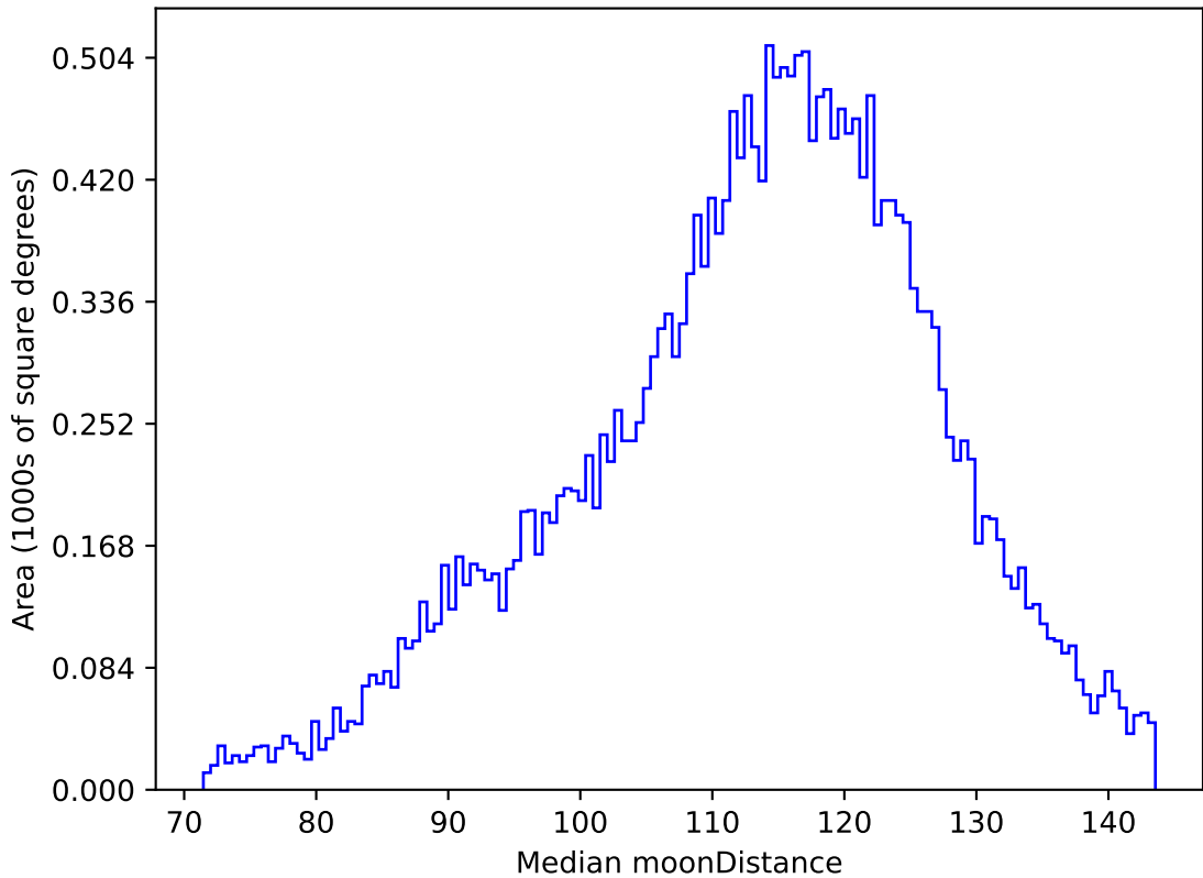
too_elab_r64_d3_gz_v3.4_10yrs All sky g band: Median moonDistance
