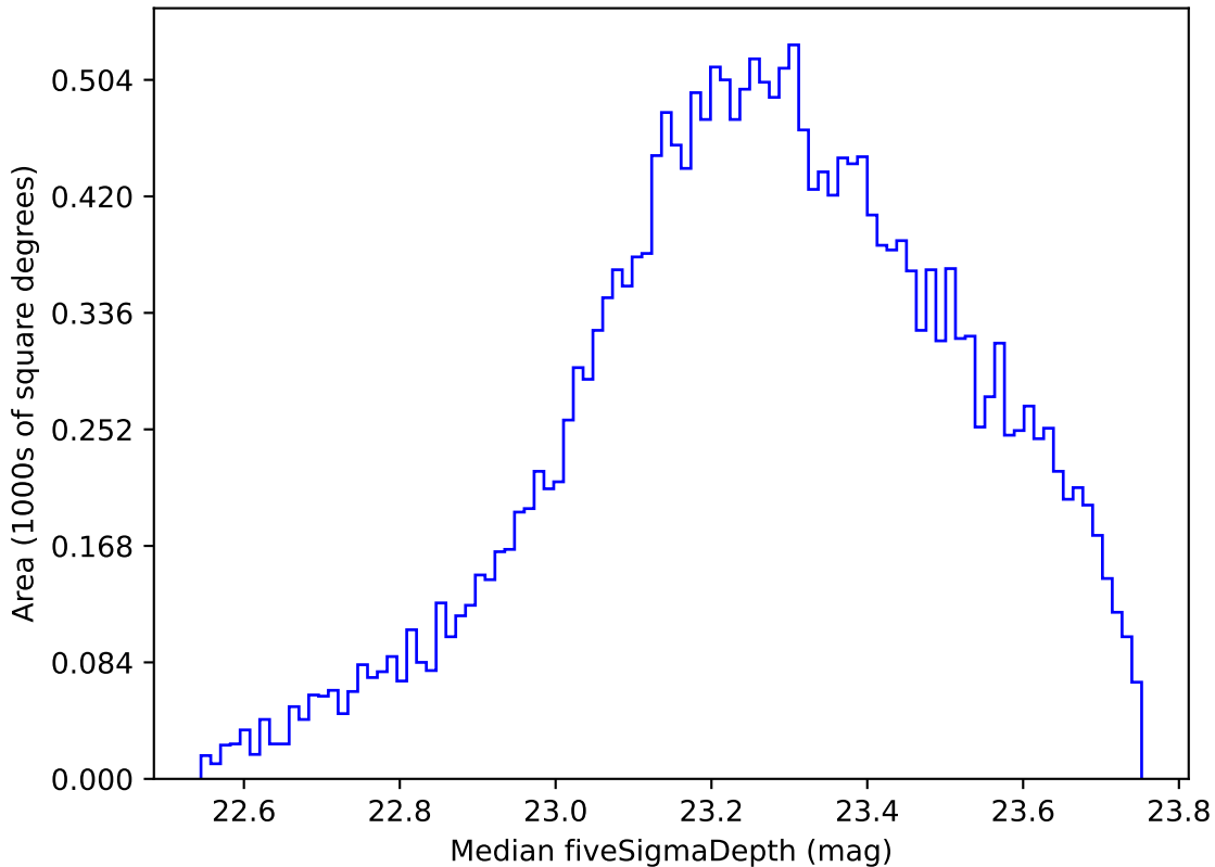
too_elab_r64_d3_gz_v3.4_10yrs Yr 1 u band: Median fiveSigmaDepth
