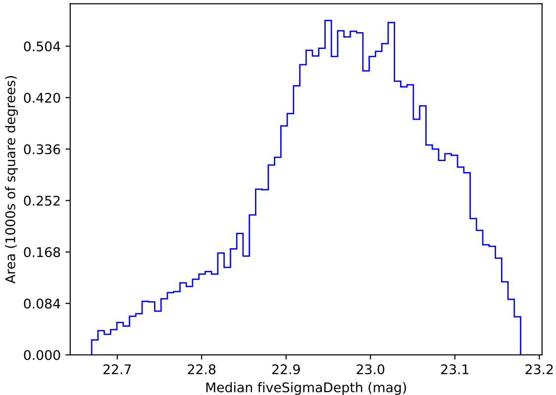
too_elab_r64_d3_gz_v3.4_10yrs WFD z band: Median fiveSigmaDepth
