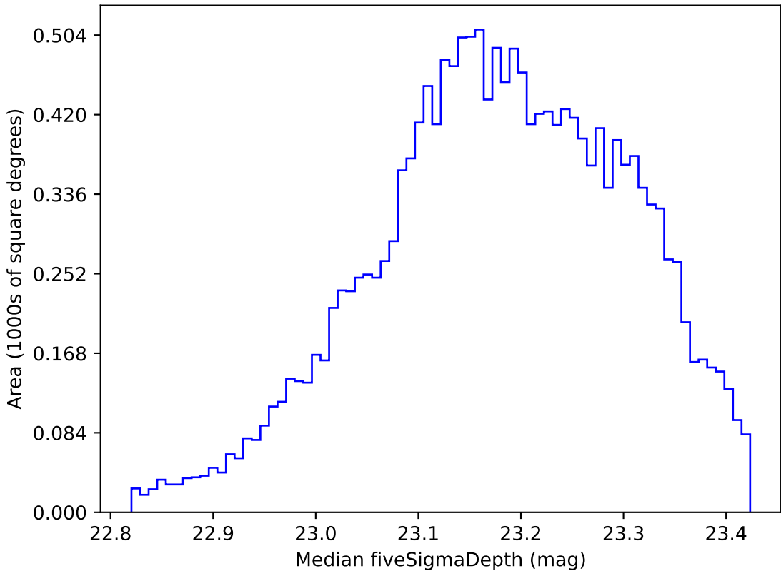
too_elab_r64_d3_gz_v3.4_10yrs WFD u band: Median fiveSigmaDepth
