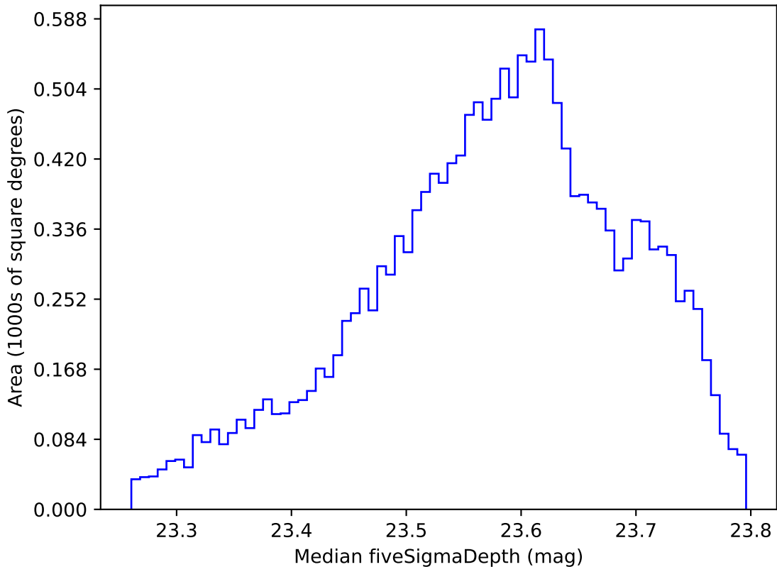
too_elab_r64_d3_gz_v3.4_10yrs WFD i band: Median fiveSigmaDepth
