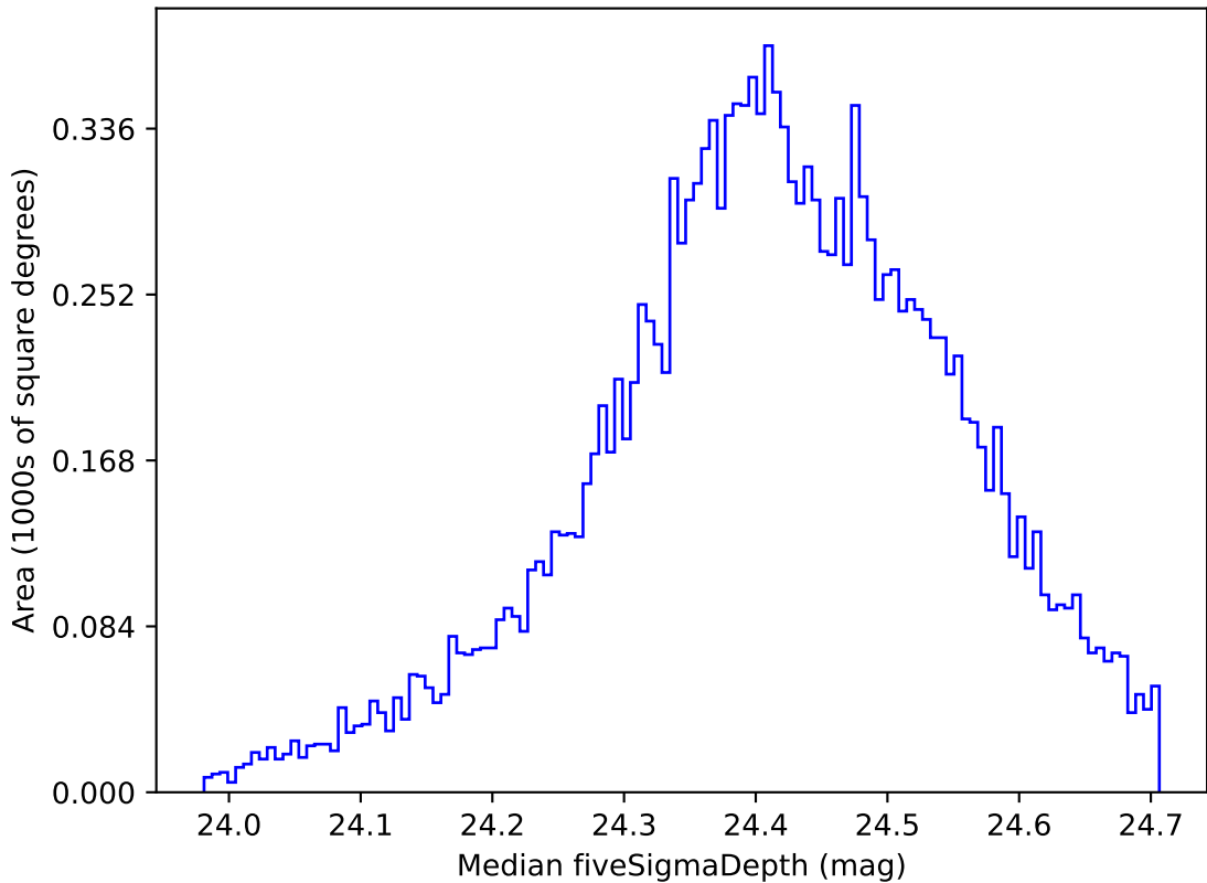
too_elab_r64_d3_gz_v3.4_10yrs WFD g band: Median fiveSigmaDepth
