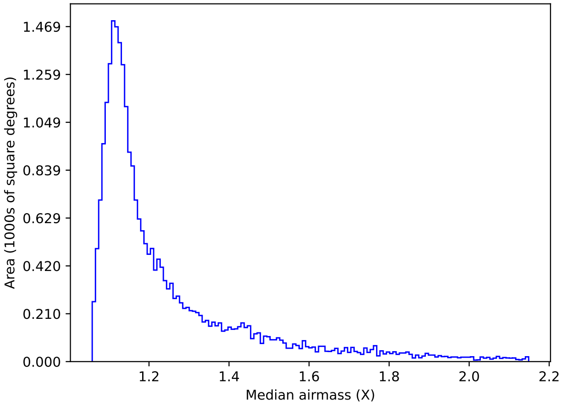
too_elab_r64_d3_gz_v3.4_10yrs Yr 1 z band: Median airmass
