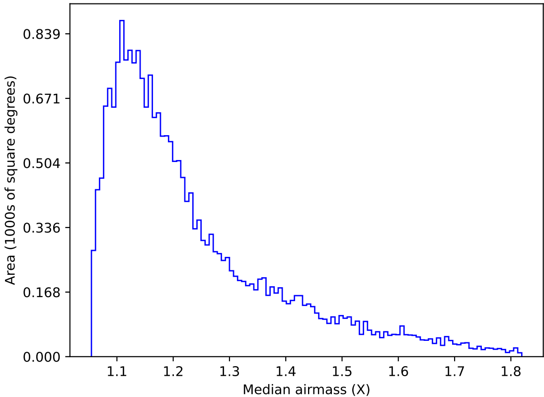
too_elab_r64_d3_gz_v3.4_10yrs Yr 1 u band: Median airmass
