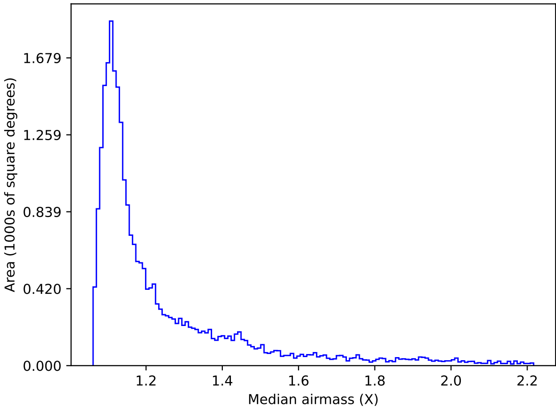
too_elab_r64_d3_gz_v3.4_10yrs Yr 1 i band: Median airmass
