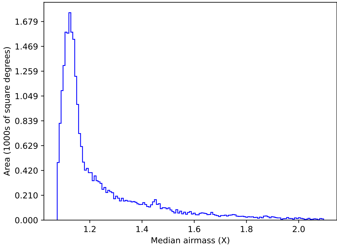
too_elab_r64_d3_gz_v3.4_10yrs Yr 1 all bands: Median airmass
