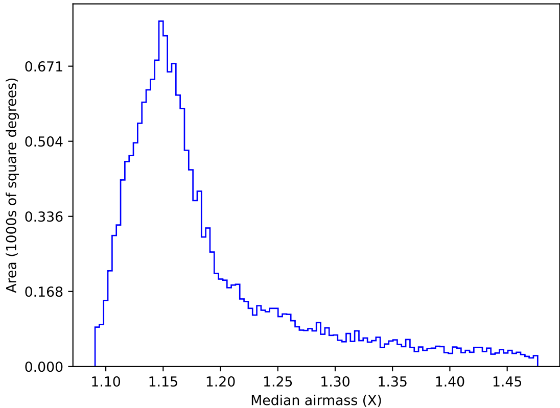
too_elab_r64_d3_gz_v3.4_10yrs WFD z band: Median airmass
