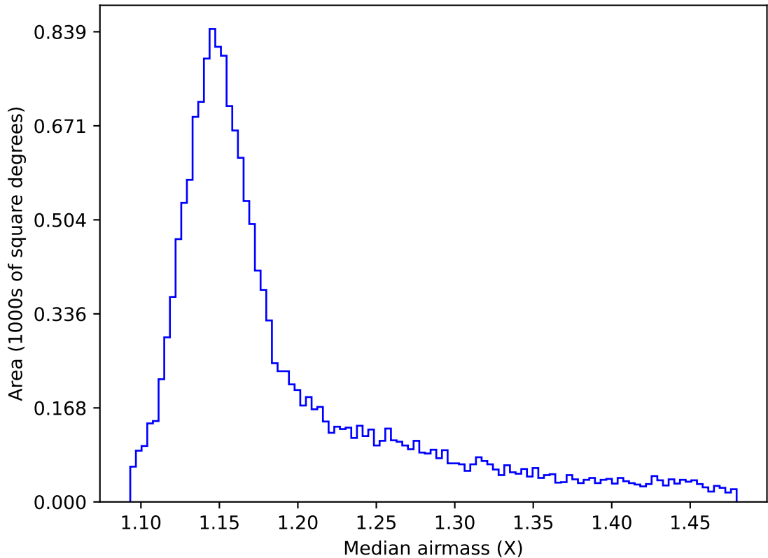
too_elab_r64_d3_gz_v3.4_10yrs WFD y band: Median airmass
