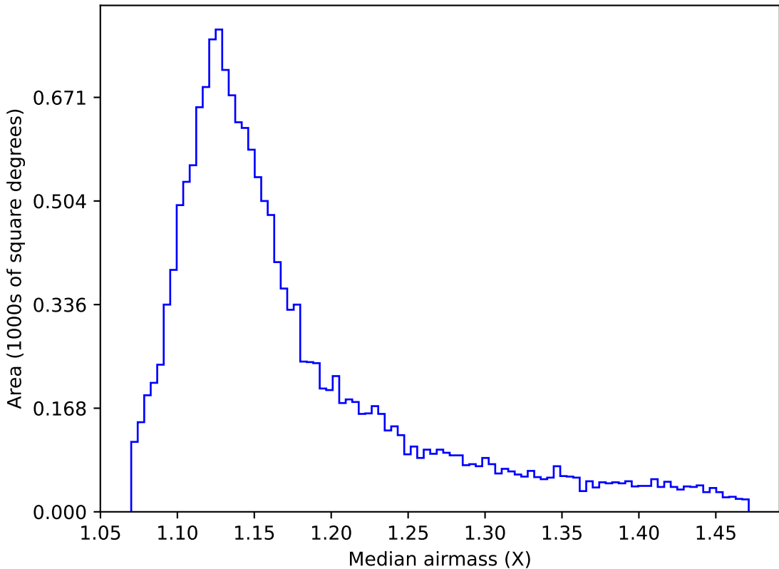
too_elab_r64_d3_gz_v3.4_10yrs WFD u band: Median airmass
