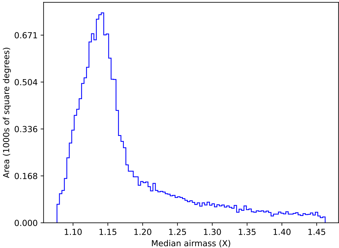
too_elab_r64_d3_gz_v3.4_10yrs WFD i band: Median airmass
