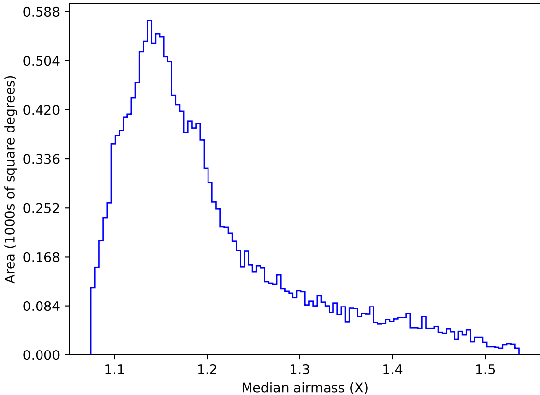
too_elab_r64_d3_gz_v3.4_10yrs WFD g band: Median airmass
