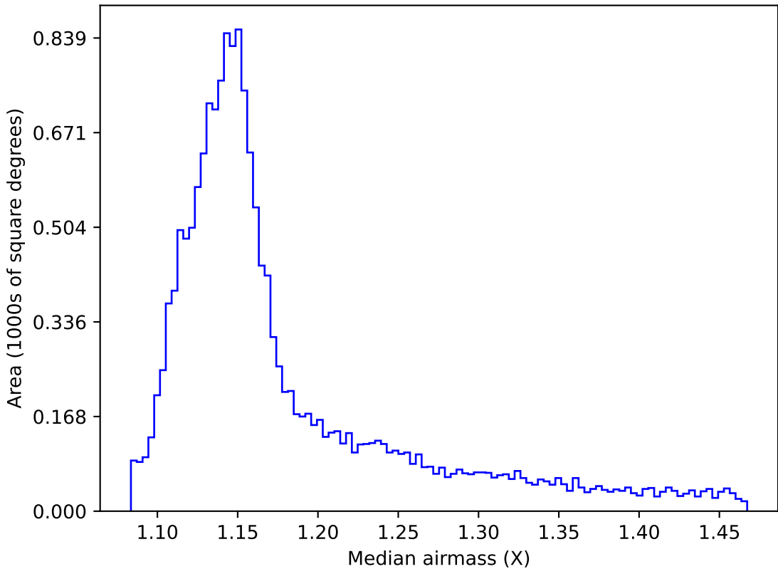
too_elab_r64_d3_gz_v3.4_10yrs WFD all bands: Median airmass
