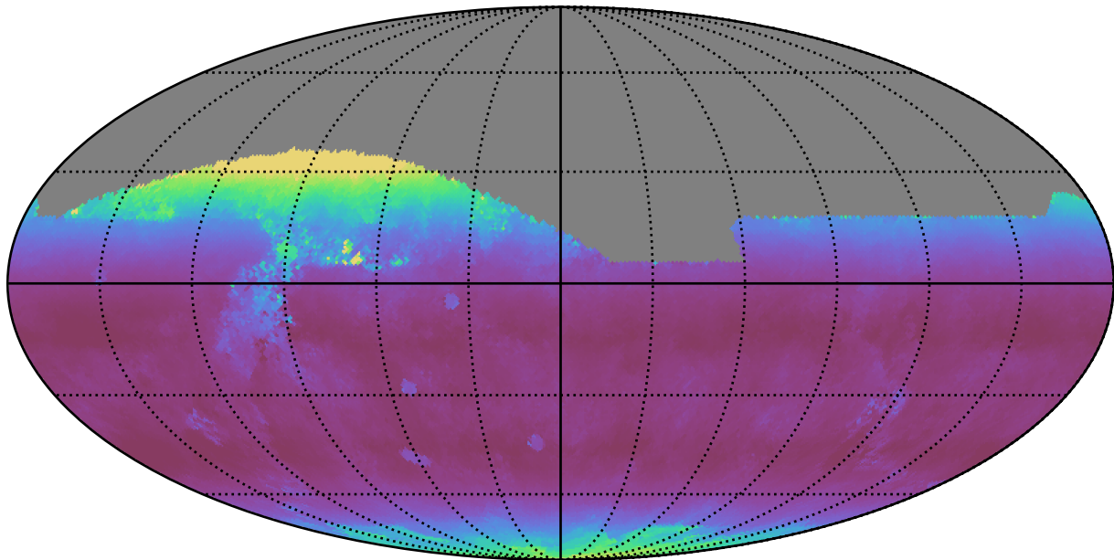
too_elab_r64_d3_gz_v3.4_10yrs All sky z band: Median airmass
