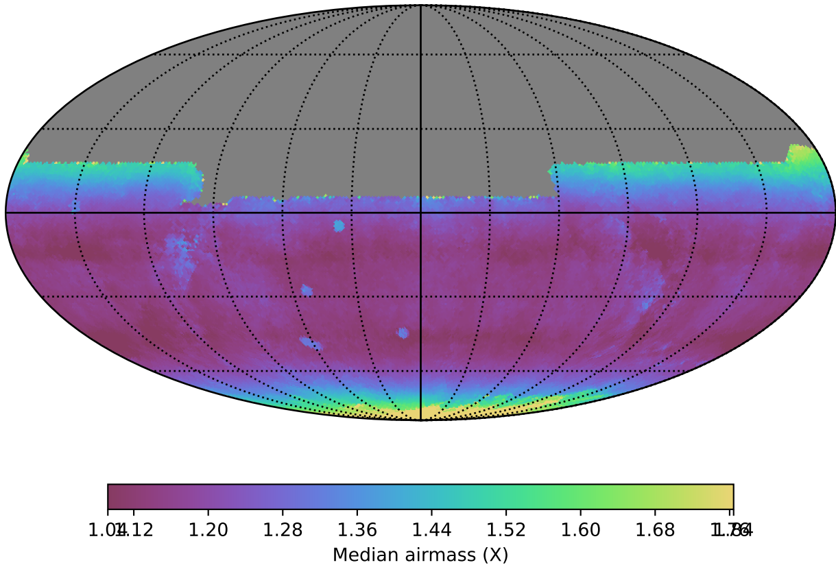
too_elab_r64_d3_gz_v3.4_10yrs All sky y band: Median airmass
