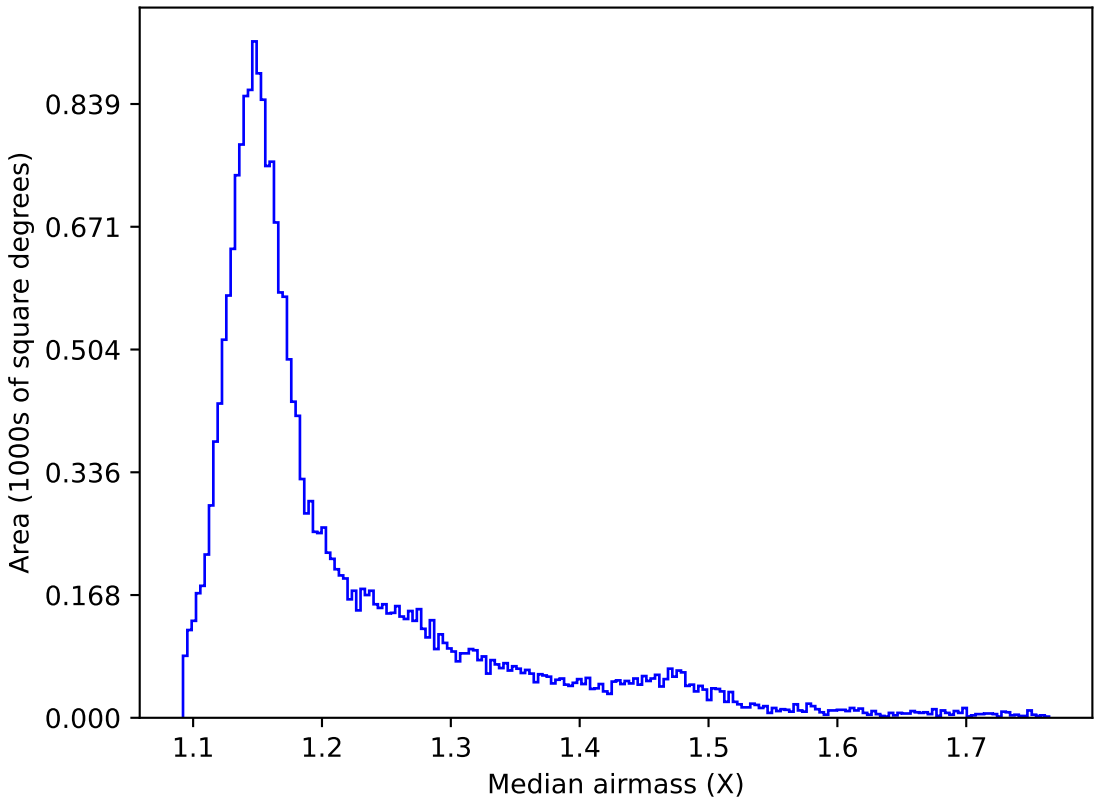
too_elab_r64_d3_gz_v3.4_10yrs All sky y band: Median airmass
