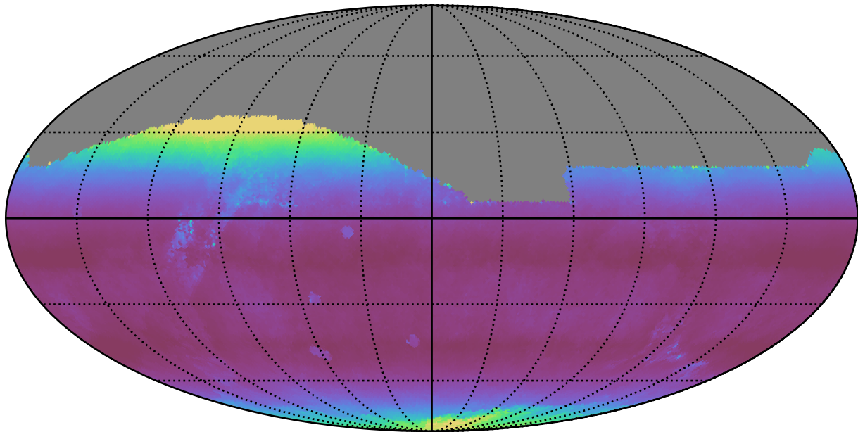
too_elab_r64_d3_gz_v3.4_10yrs All sky r band: Median airmass
