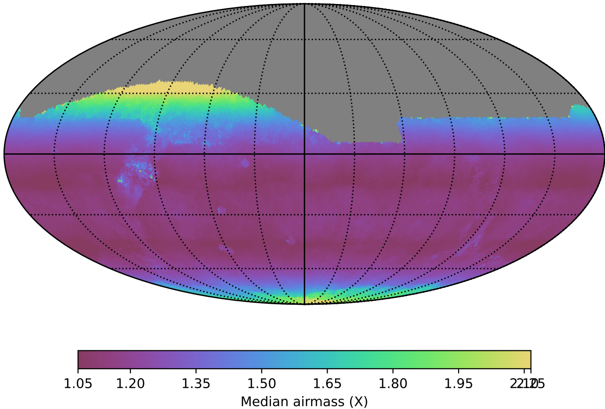
too_elab_r64_d3_gz_v3.4_10yrs All sky i band: Median airmass
