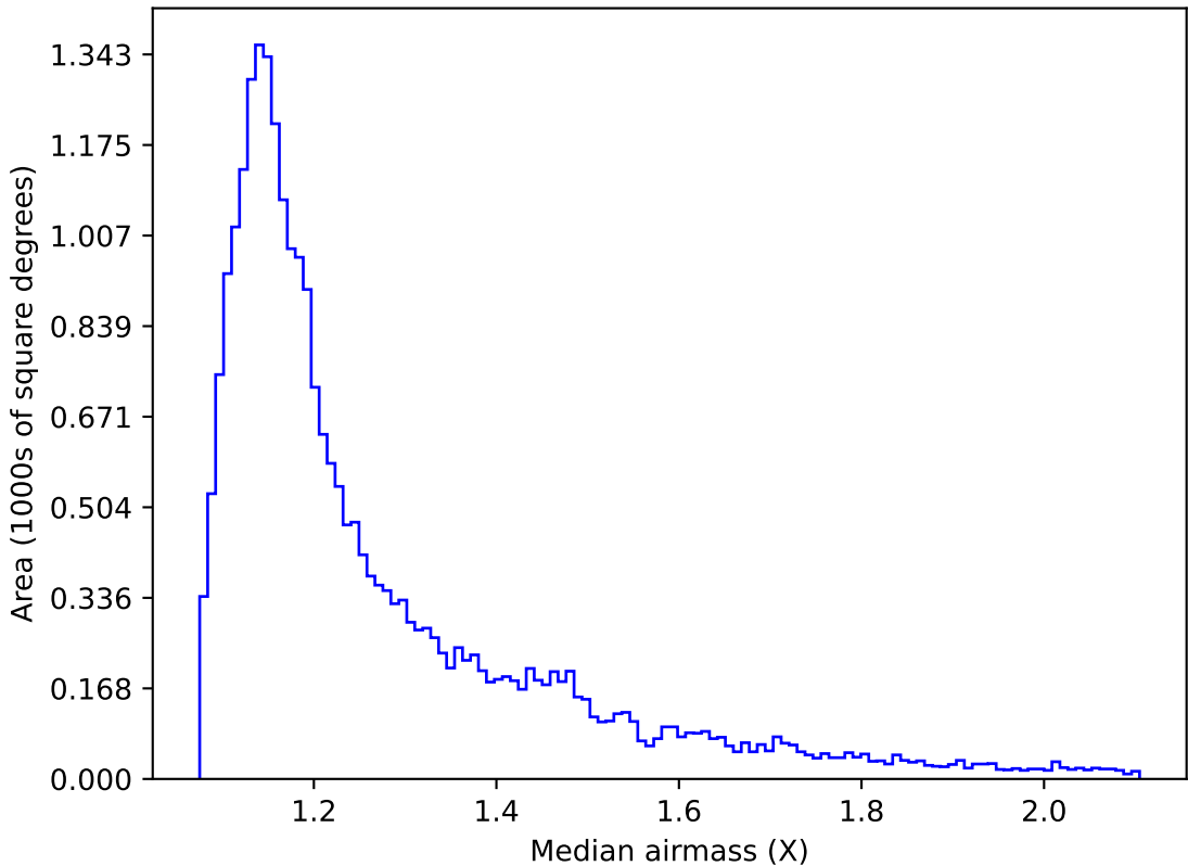
too_elab_r64_d3_gz_v3.4_10yrs All sky g band: Median airmass
