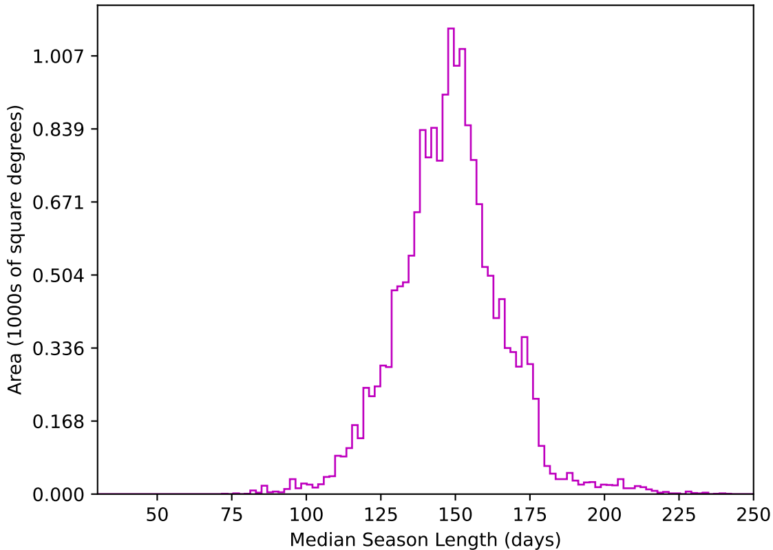
too_elab_r64_d3_gz_v3.4_10yrs WFD z band: Median Season Length
