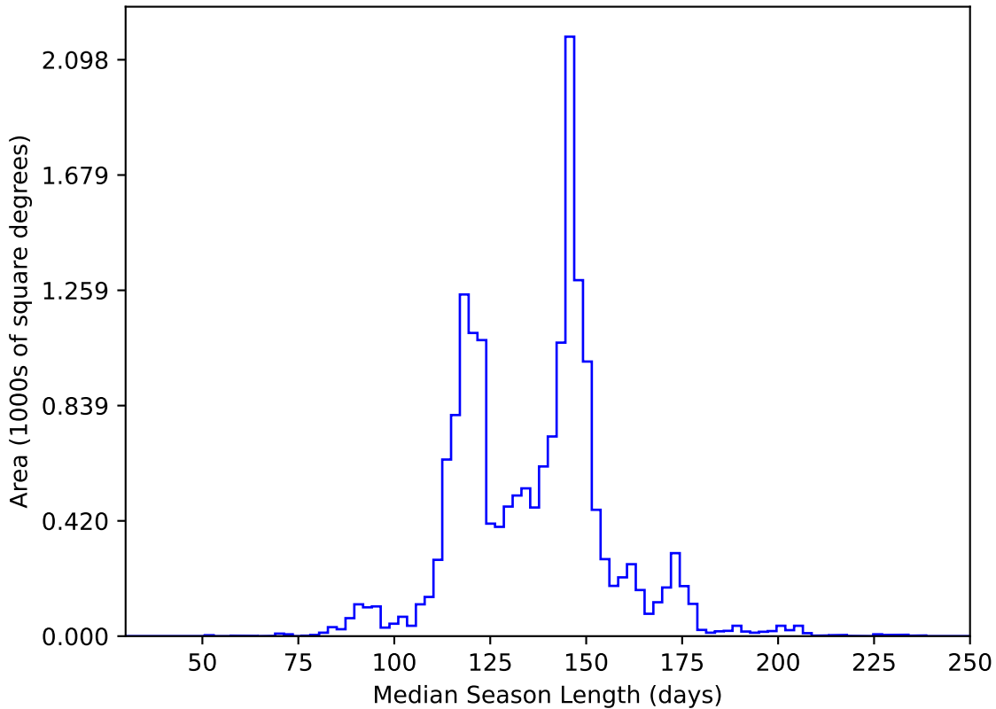
too_elab_r64_d3_gz_v3.4_10yrs WFD y band: Median Season Length
