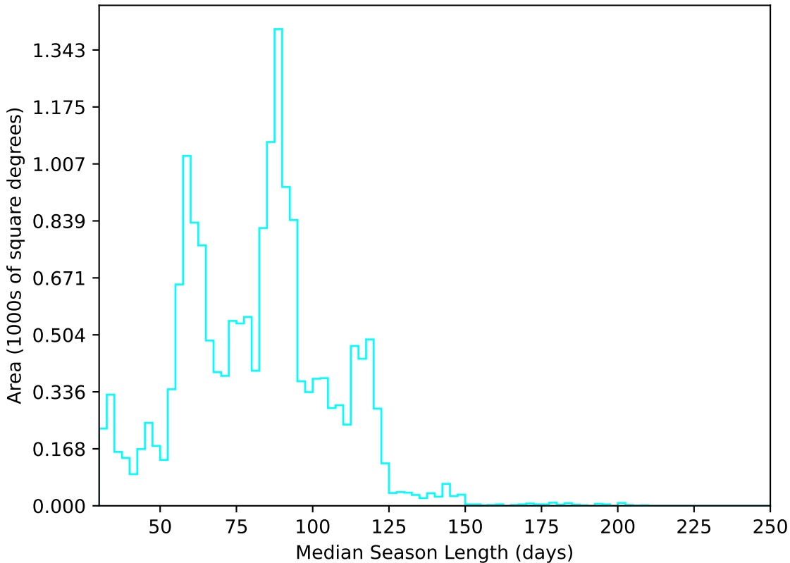
too_elab_r64_d3_gz_v3.4_10yrs WFD u band: Median Season Length
