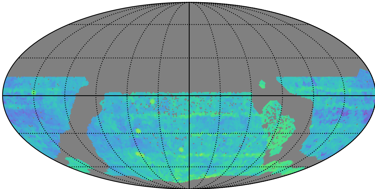
too_elab_r64_d3_gz_v3.4_10yrs WFD r band: Median Season Length
