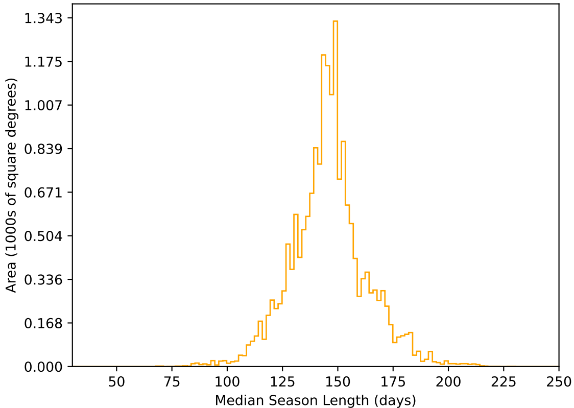
too_elab_r64_d3_gz_v3.4_10yrs WFD r band: Median Season Length
