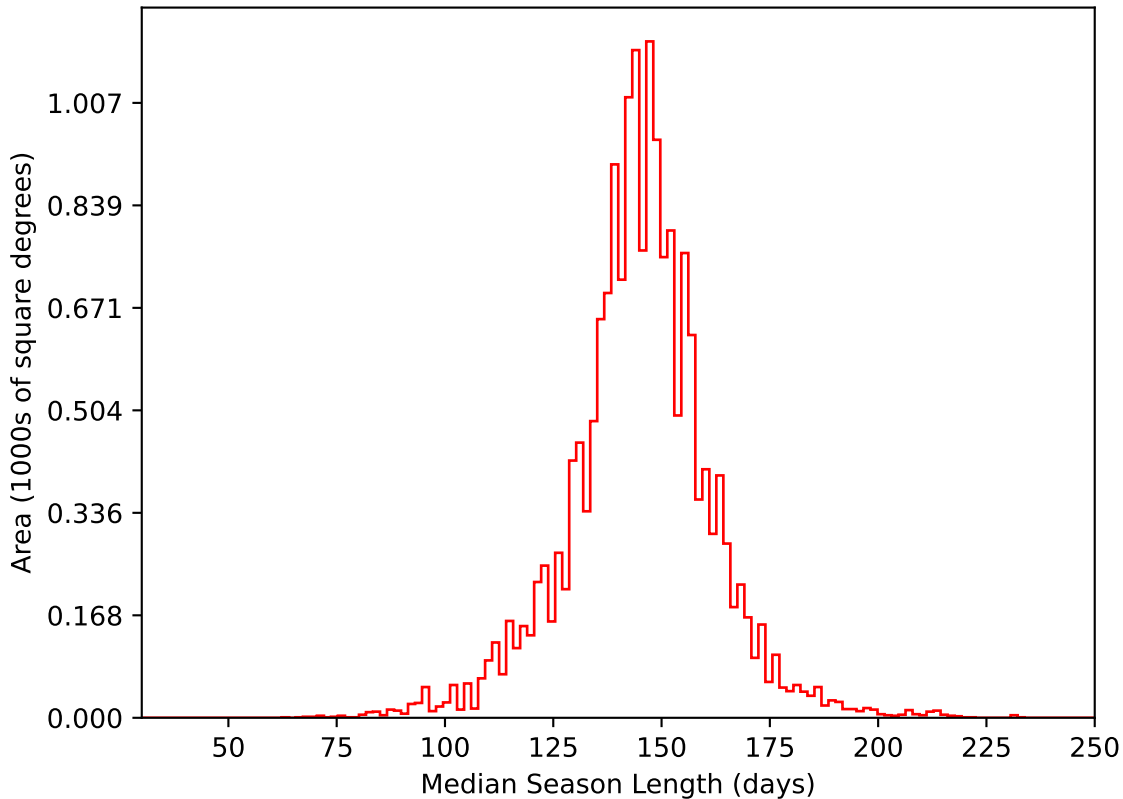
too_elab_r64_d3_gz_v3.4_10yrs WFD i band: Median Season Length
