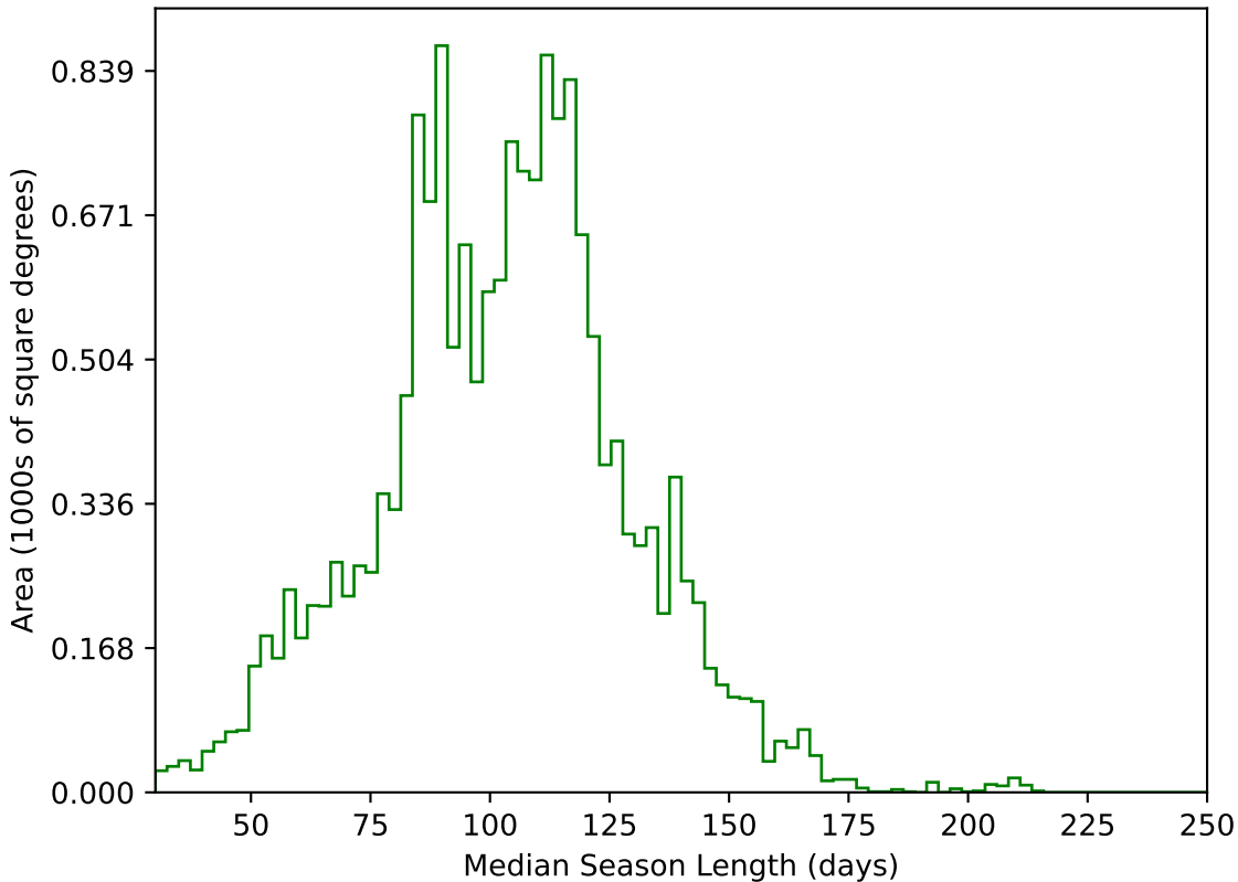
too_elab_r64_d3_gz_v3.4_10yrs WFD g band: Median Season Length
