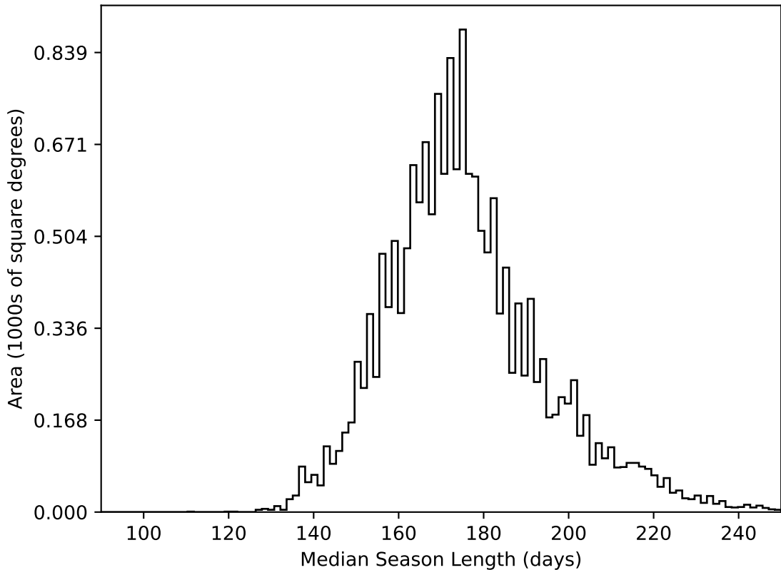
too_elab_r64_d3_gz_v3.4_10yrs WFD all bands: Median Season Length
