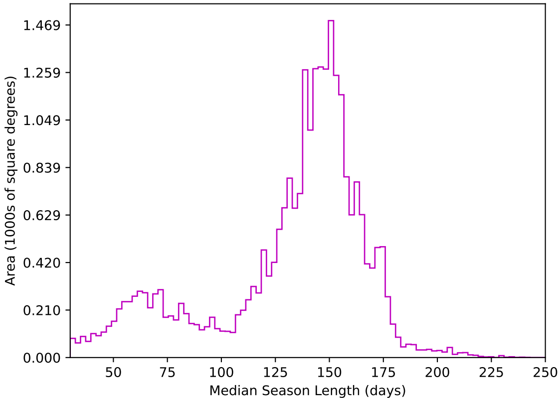
too_elab_r64_d3_gz_v3.4_10yrs All sky z band: Median Season Length
