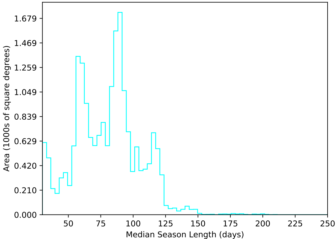
too_elab_r64_d3_gz_v3.4_10yrs All sky u band: Median Season Length
