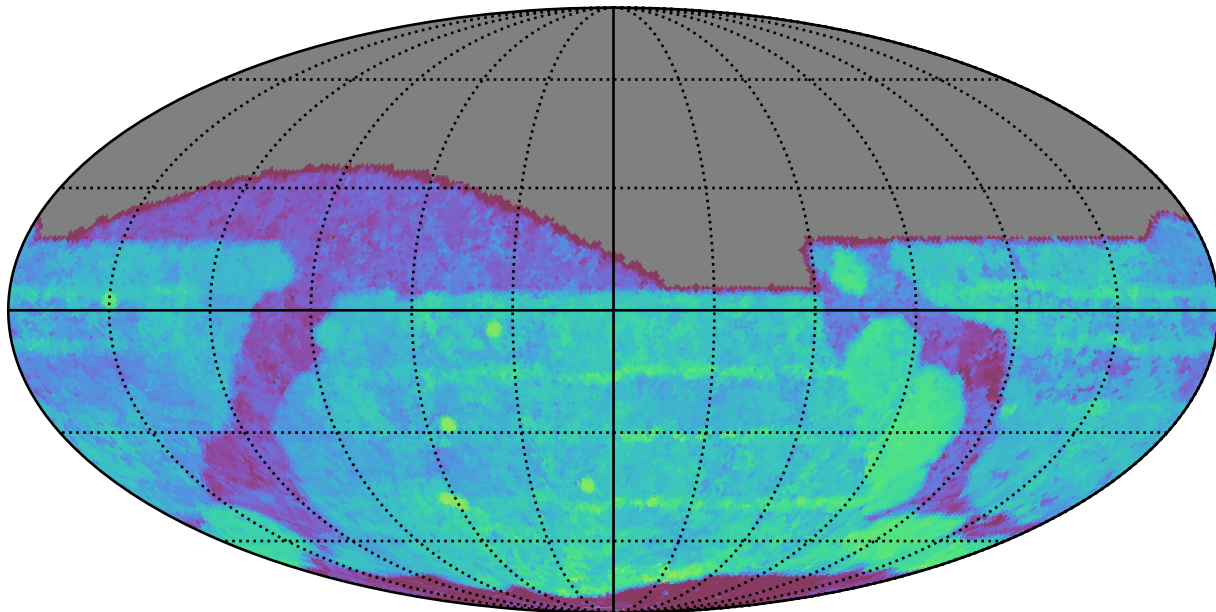
too_elab_r64_d3_gz_v3.4_10yrs All sky r band: Median Season Length
