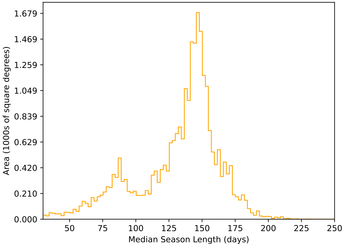
too_elab_r64_d3_gz_v3.4_10yrs All sky r band: Median Season Length
