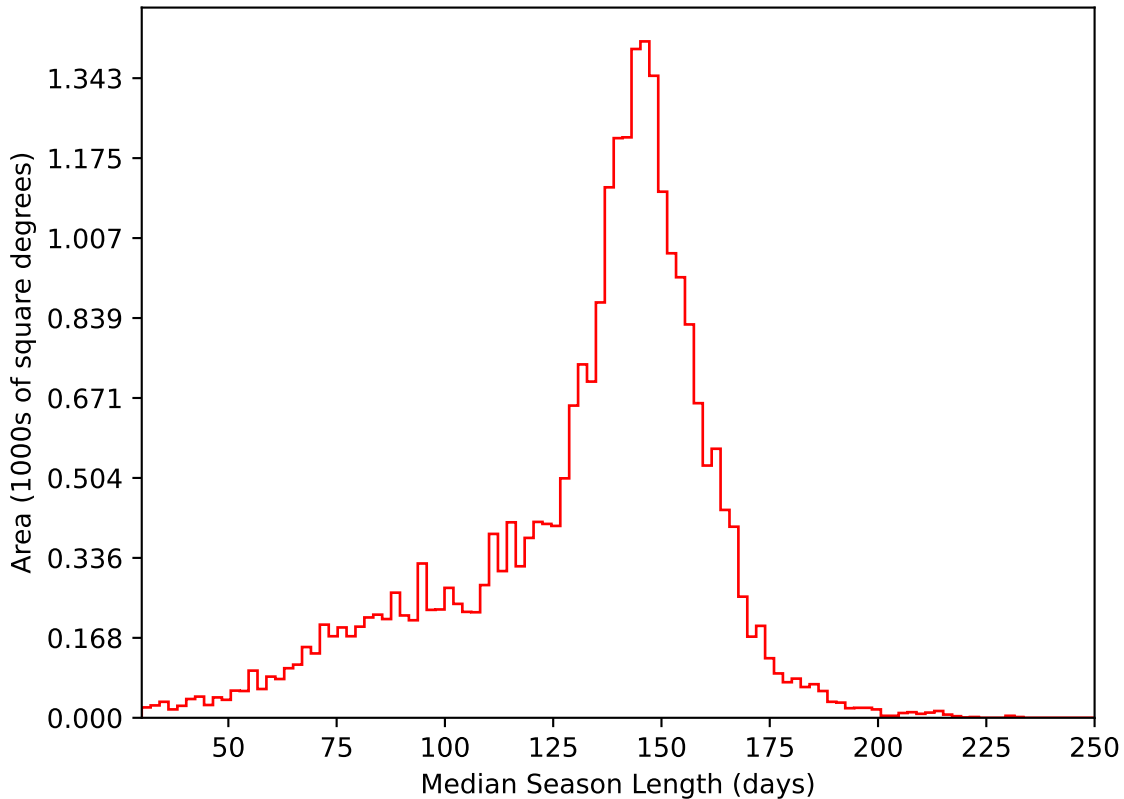
too_elab_r64_d3_gz_v3.4_10yrs All sky i band: Median Season Length
